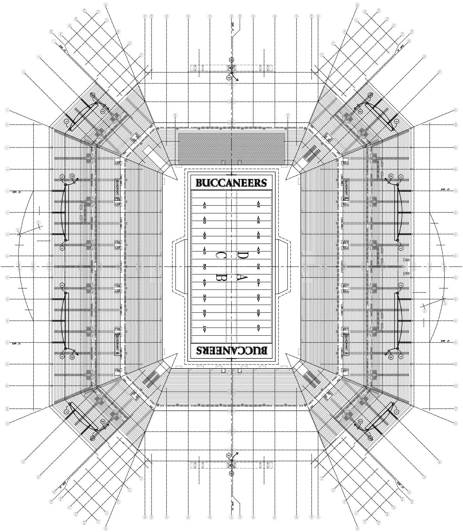
NEW WORK OBSTRUCTION LIGHTING PLAN SCALE: 1"=40'-0"
