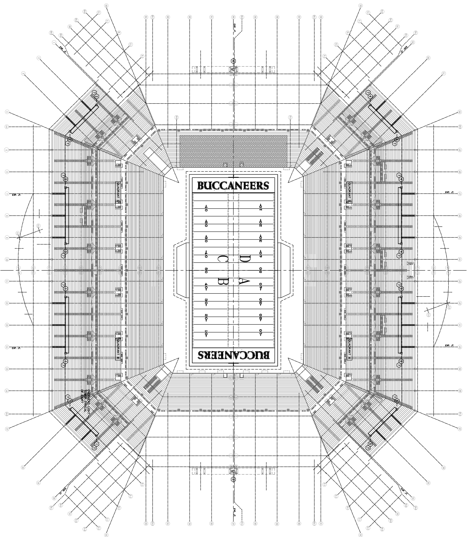
ELECTRICAL DEMOLITION PLAN SCALE: 1"=40'-0" 7/11/17
