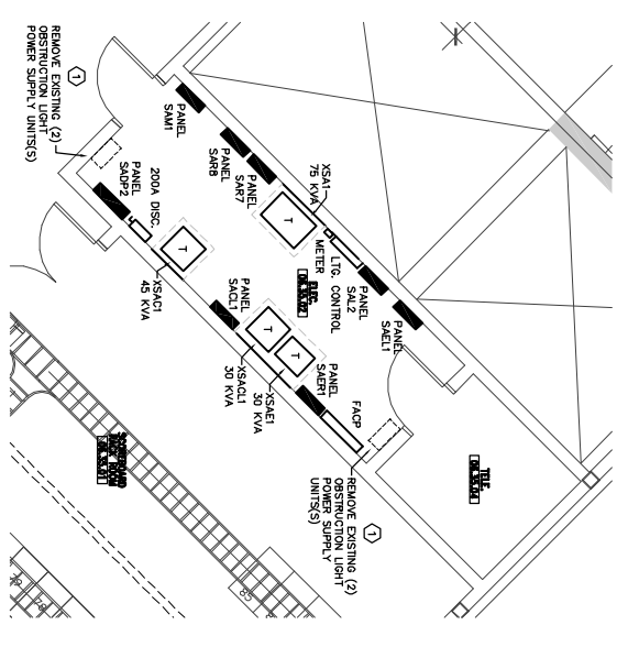
QUADRANT "A" ELECTRICAL ROOM. SCALE: 1/4"=1'-0" 14147
