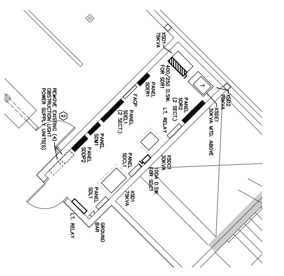
QUADRANT "D" ELECTRICAL ROOM. SCALE: 1/4"=1'-0" 14147
