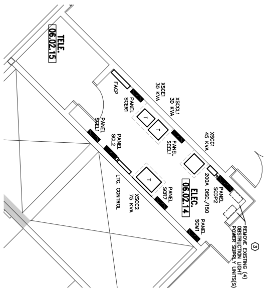
QUADRANT "C" UPPER SUITE ELECTRICAL ROOM. SCALE: 1/4"=1'-0" 14147
